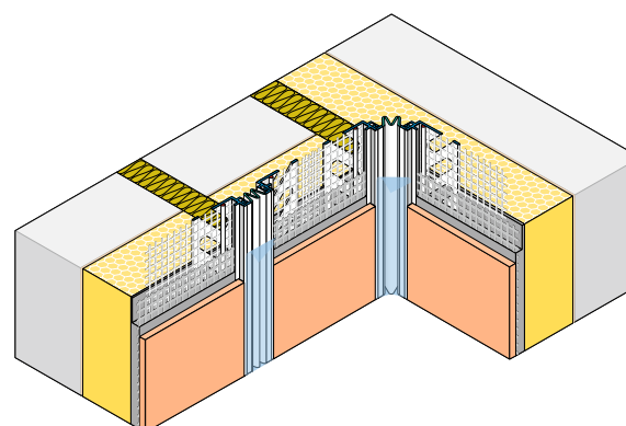
Application drawing
